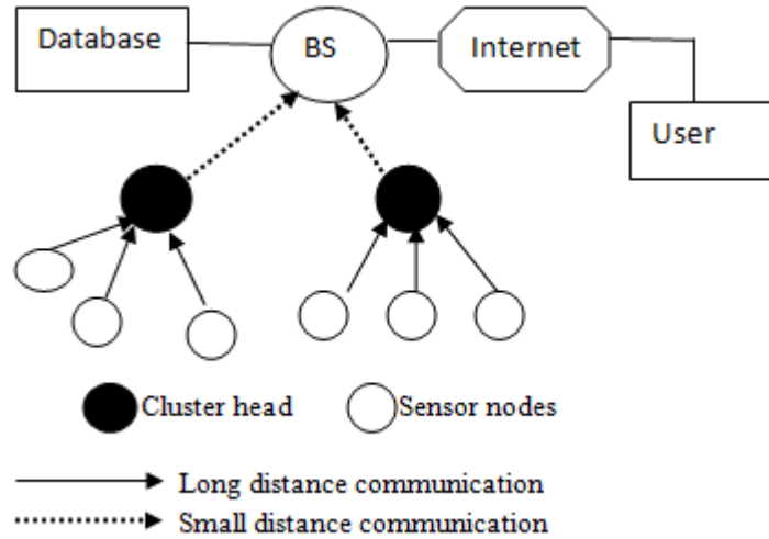
Fig.1. Clustering technique
